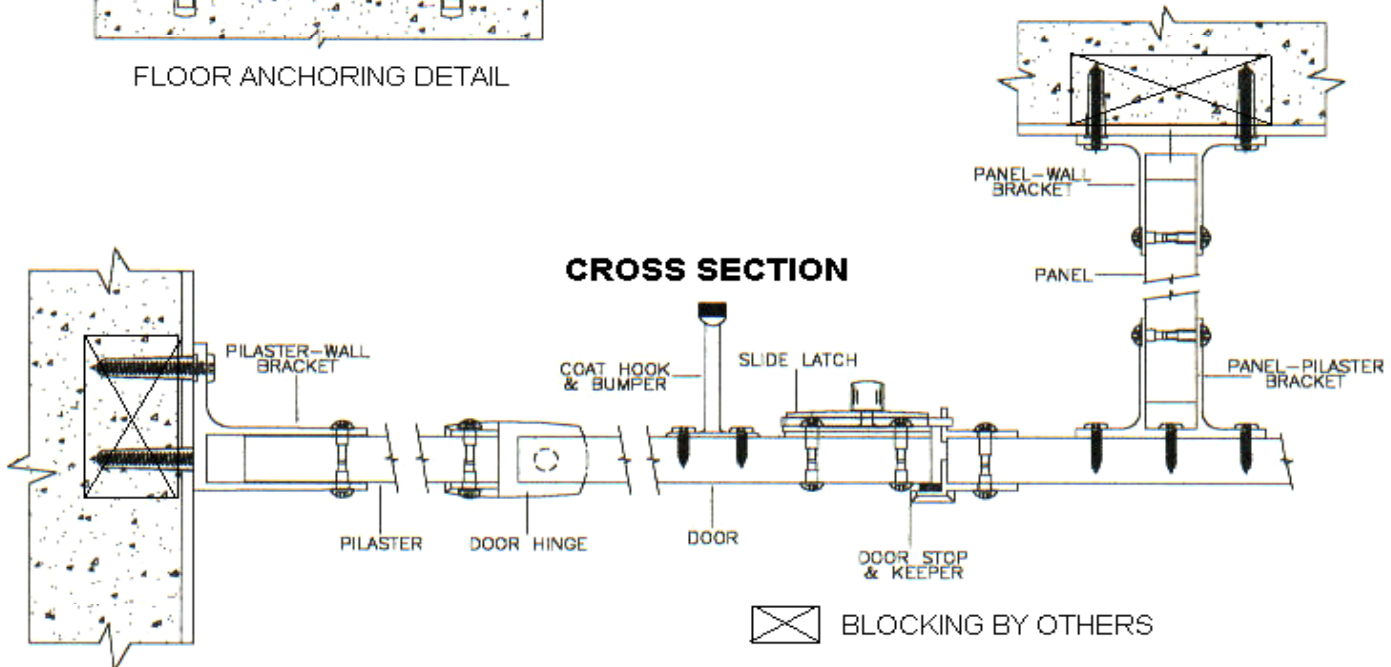
HEADRAIL DETAIL
