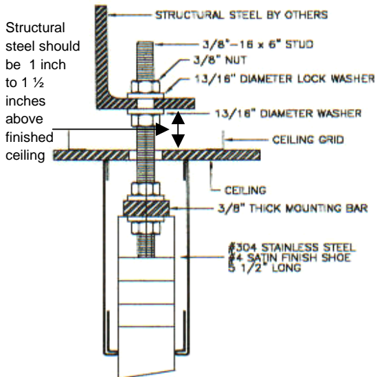
CEILING BOLT DETAIL
