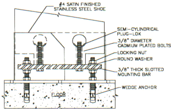
FLOOR ANCHORING DETAIL
