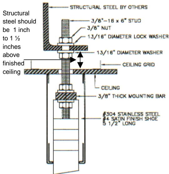
CEILING BOLT DETAIL
